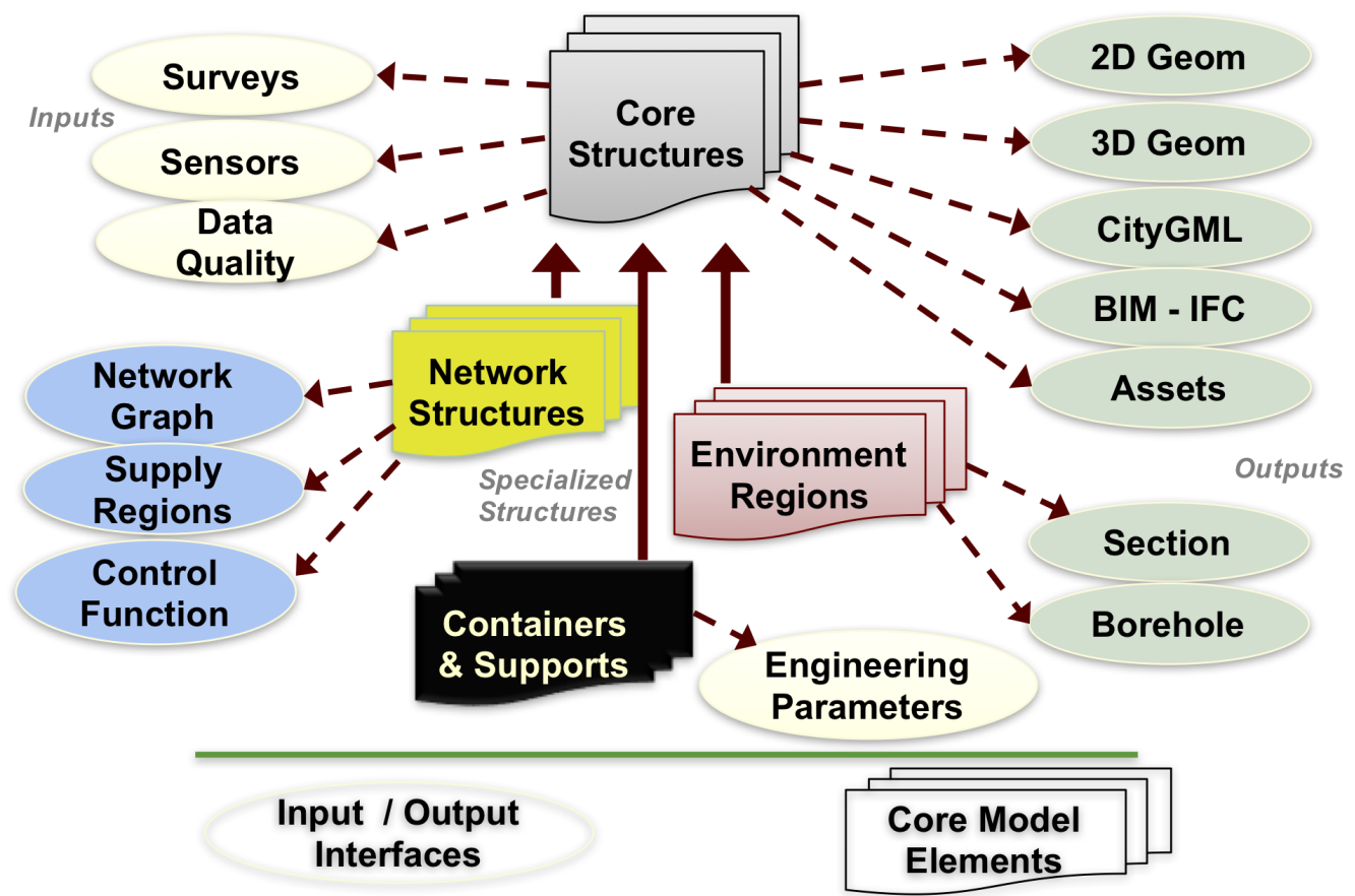
Figure 9. MUDDI
